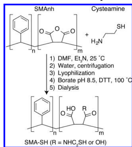
Scheme 1. Reaction Scheme for the Preparation of SMA-SH
