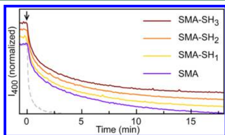
Figure 2. Liposome dissolution by SMA-SH x and SMA proceeds identically. The intensity of 400 nm light scattered by a solution of 0.05 mg/mL DMPC liposomes at 20 °C diminishes upon addition of up to 0.15 mg/mL SMA or SMA-SH x at t = 0 (indicated with an arrow). Each curve is normalized to the initial intensity and offset to facilitate comparison. The dashed gray line shows diminishing of light scattering upon addition of SMA at 25 °C.
