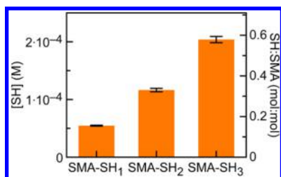
Figure 1. Ratio of SMAnh to cysteamine used in the reaction tunes the amount of sulfhydryls in SMA-SH. The concentration of sulfhydryls in SMA-SH x solutions of 2.6 mg/mL was determined using the Ellman's assay; error bars show the standard deviation of duplicate measurements. The concentration of polymer was calculated using a molecular weight of 7500 g/mol.
