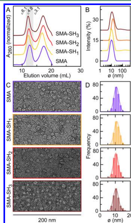
Figure 3. Like SMA, SMA-SH dissolves lipid bilayer membranes into lipid nanodiscs. (A) Elution profiles of SMA- and SMA-SH x -DMPC nanodiscs obtained by analytical size-exclusion chromatography on a Superdex 200 Increase column. Numbers above the chromatograms indicate hydrodynamic radii ( R_H ; nm) corresponding to calibration standards. R_H of the majority of lipid nanodiscs ranges from 3.6 and 5.3 nm (indicated by the gray area). (B) Intensity-based particle diameter distributions, obtained from DLS analysis of SMA- and SMA-SH x -DMPC nanodiscs eluting between 12.3 and 12.8 mL. Average particle diameters and corresponding standard deviations are 11.1 \pm 4.0 , 10.9 \pm 3.6 , 14.8 \pm 5.0 , and 13.5 \pm 6.2 nm for SMA, SMA-SH 1 , SMA-SH 2 , and SMA-SH 3 , respectively. (C) Representative negative stain transmission electron micrograph of SMA- and SMA-SH x -DMPC nanodiscs. (D) TEM-based particle diameter distributions, obtained from measurement of 200 particles. Average particle diameters and corresponding standard deviations are 10.0 \pm 1.6 , 10.5 \pm 2.0 , 9.7 \pm 1.6 , and 10.1 \pm 2.0 nm for SMA-, SMA-SH 1 -, SMA-SH 2 -, and SMA-SH 3 -DMPC nanodiscs, respectively. Dotted lines represent the fit of a Gaussian distribution to the data.
