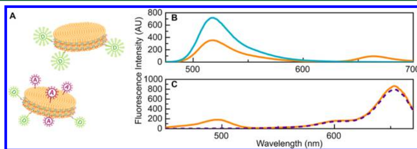
Figure 5. SMA-SH-lipid nanodiscs sustain covalent modification of sulfhydryls on the polymer that surrounds them. (A) Schematic representation of A488-labeled SMA-SH-DMPC nanodiscs in absence and presence of Atto647N-labeled DMPE (top and bottom, respectively). The donor and acceptor dyes are labeled with D and A, respectively. (B) Emission spectrum of A488-labeled SMA-SH-DMPC nanodiscs (cyan line) and A488-labeled SMA-SH 3 -[DMPC + 1% Atto647N-DMPE] nanodiscs (orange line), upon excitation at 465 nm. (C) Excitation spectrum of A488-labeled SMA-SH 3 -[DMPC + 1% Atto647N-DMPE] nanodiscs (orange line) and SMA-[DMPC + 1% Atto647N-DMPE] nanodiscs (dashed purple line), monitored at 680 nm.
